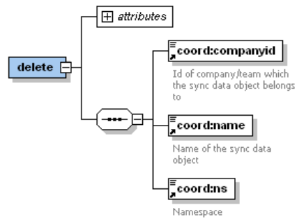
Figure – Schema – delete syncdata operation
